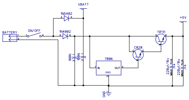
ICHIBOT ULTIMATE 3 DIP REFERENCE DESIGN WWW.TEAM-ICHIBOT.ID ©2018
